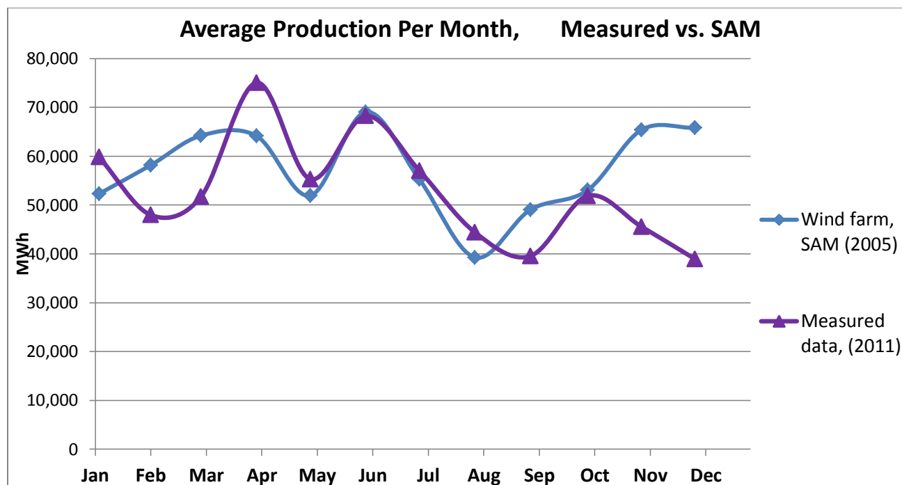
Figure 16. Average electricity production per month. Measured vs. Wind farm (2005) in SAM
