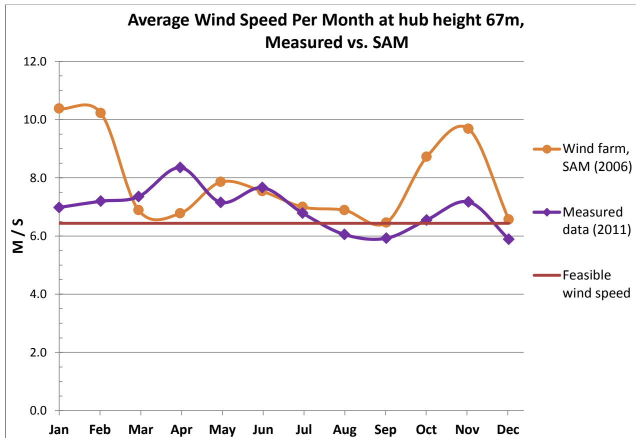
Figure A - 3. Average wind speed per month at hub height (67 meters). Measured vs. location (2006) in SAM.
