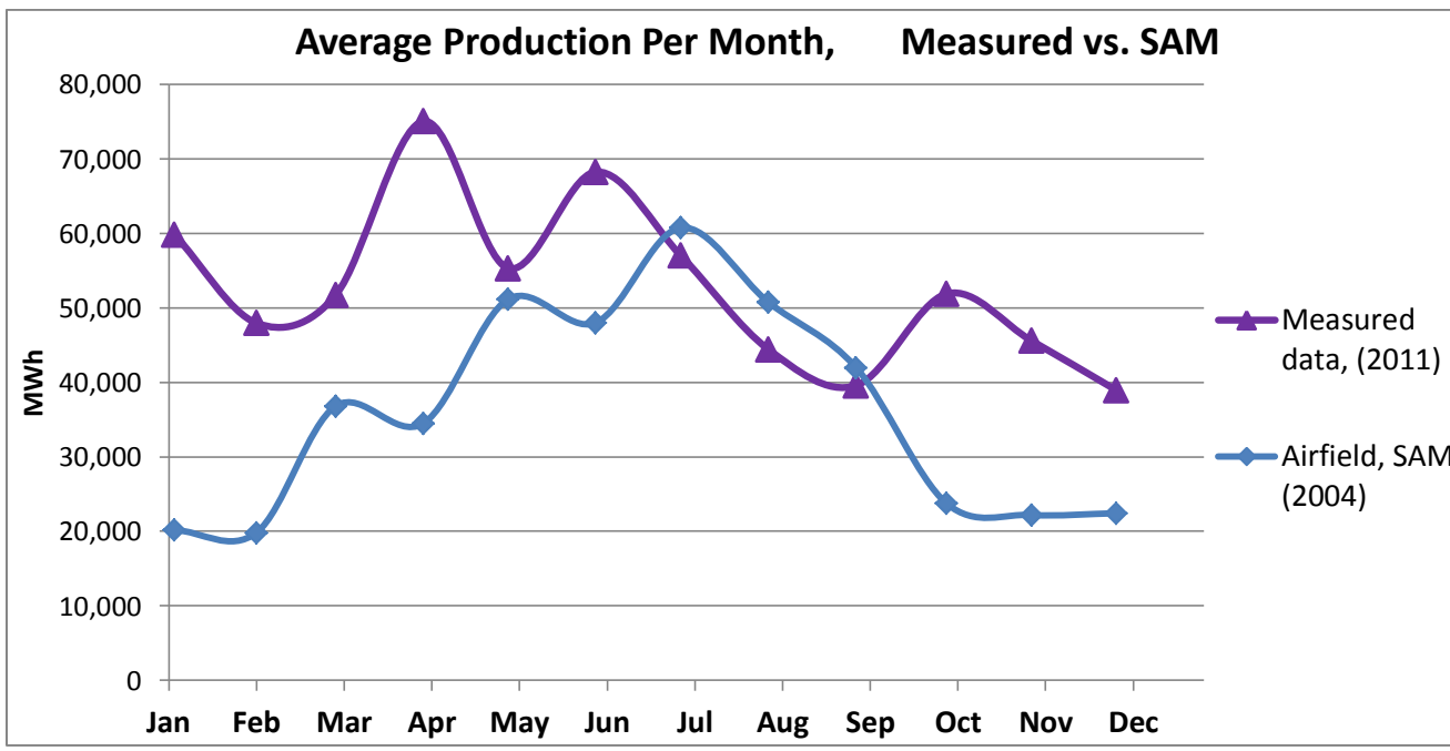
Figure B - 4. Average electricity production per month. Measured vs. Airfield (2004) in SAM
